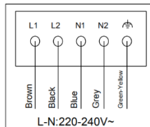
API2300I
